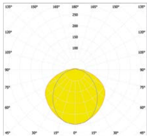
POLAR DIAGRAM TPN | FROSTED
