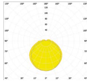
POLAR DIAGRAM TPN | OPAL
